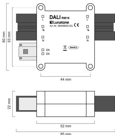
Geometrie RM16-CEL
